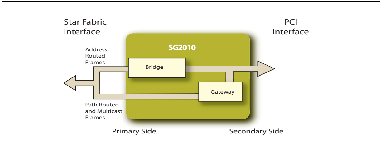
4–3 SG2010 Leaf mode with Bridge function enabled diagram
