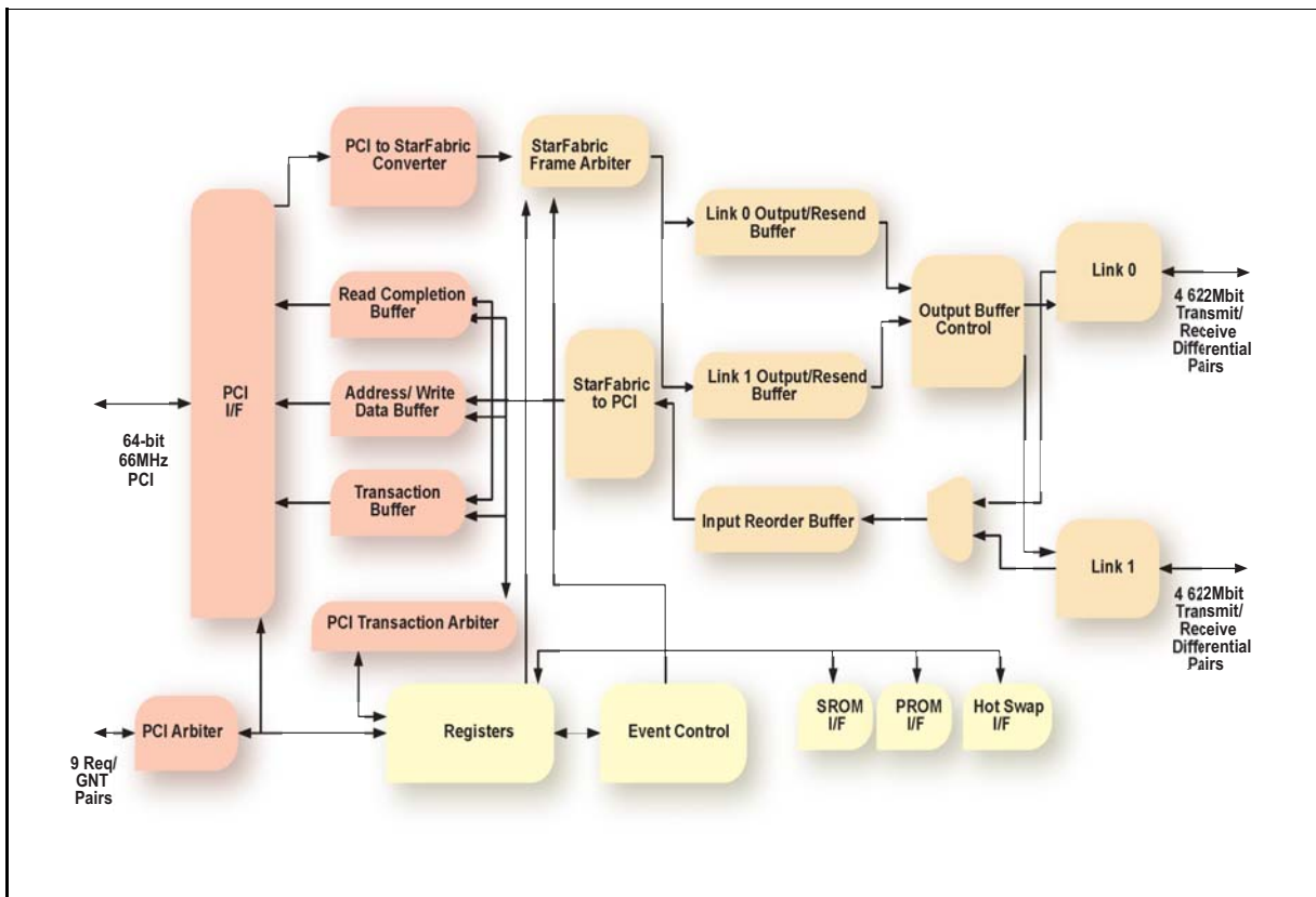
4-1 SG2010 Block Diagram
