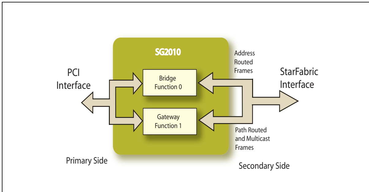
4-2 SG2010 Root Mode with Bridge function enabled diagram
